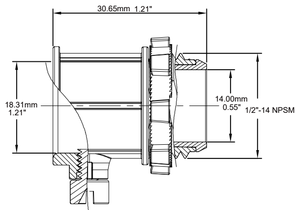
Straight joint:
