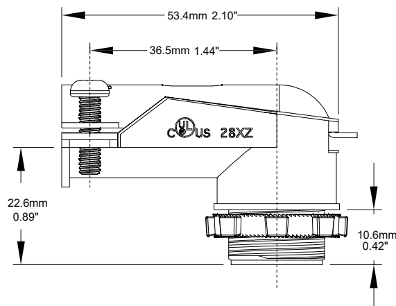
L type joint:
